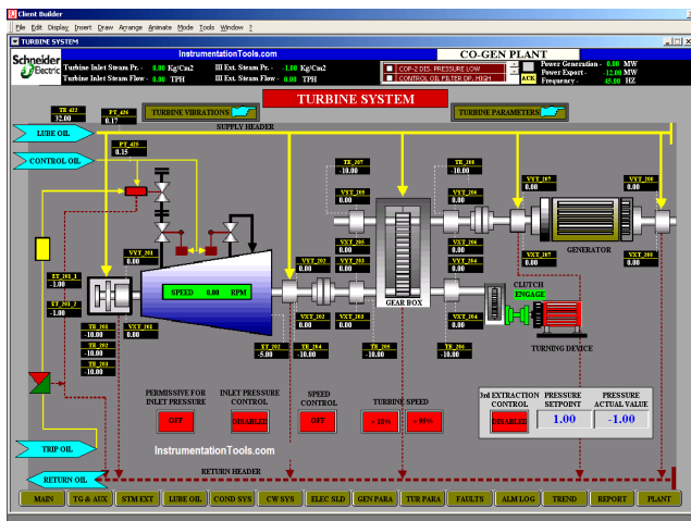
SCADA SYSTEM
